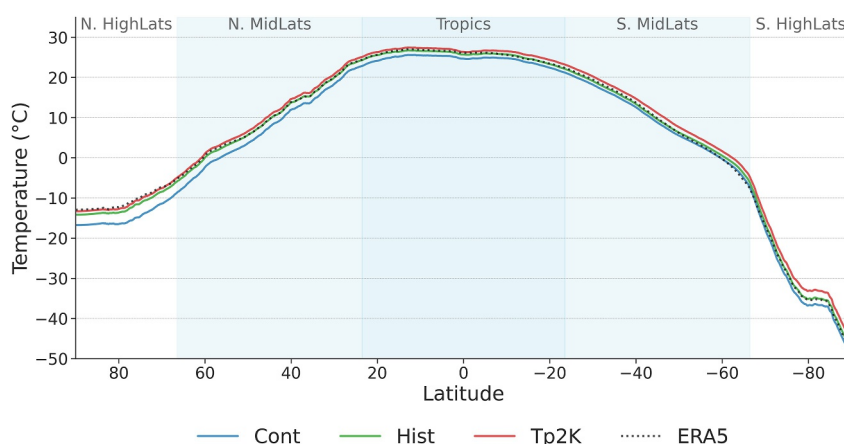
Figure 2. Zonal-mean 2 m-temperature (°C) averaged over 2018–2024 from three IFS–FESOM experiments, compared with ERA5 reanalysis. ERA5 is shown as a dotted line; IFS–FESOM results are shown for the control (Cont, blue), historical (Hist, green), and +2 K (Tp2K, red) simulations. Differences between the experiments reflect shifts in background climate conditions under different forcings, illustrating the model's sensitivity to imposed climate states, while part of the hemispheric contrast likely also reflects residual differences in ocean spin-up and deep-ocean adjustment.
