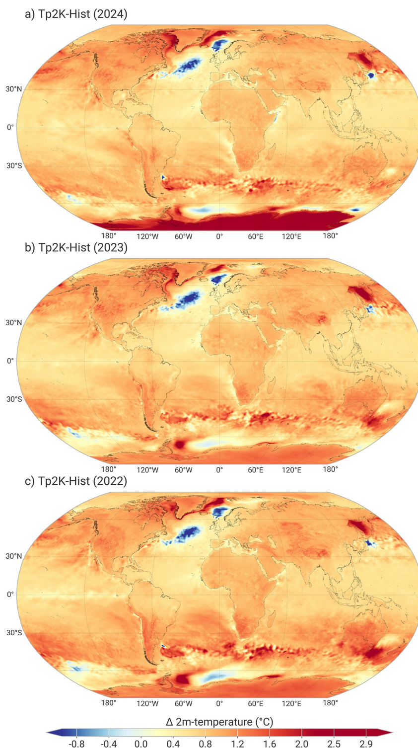
Figure 9. Maps show annual mean 2 m-temperature differences (°C) between the +2 K warmer world (Tp2K) and present-day conditions (Hist) for the years (a) 2024, (b) 2023, and (c) 2022. The comparison highlights that nudging yields spatially coherent thermodynamic signals at the annual scale. For a comparison with the single-year differences from unconstrained free-running simulations, see Figure S11 in Supporting Information S1.
